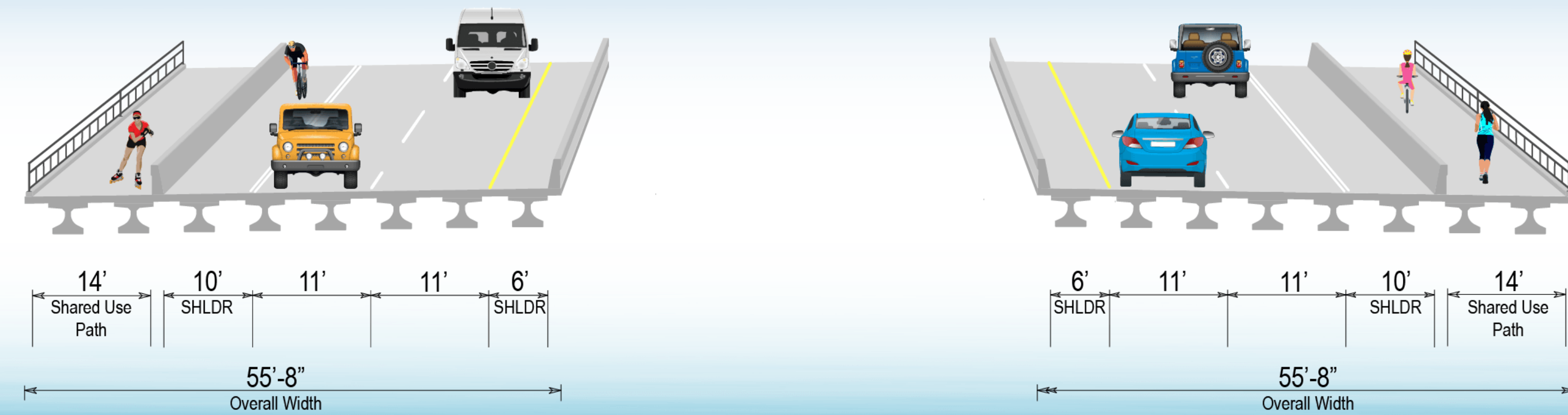
PROPOSED TWIN BRIDGE TYPICAL SECTION
