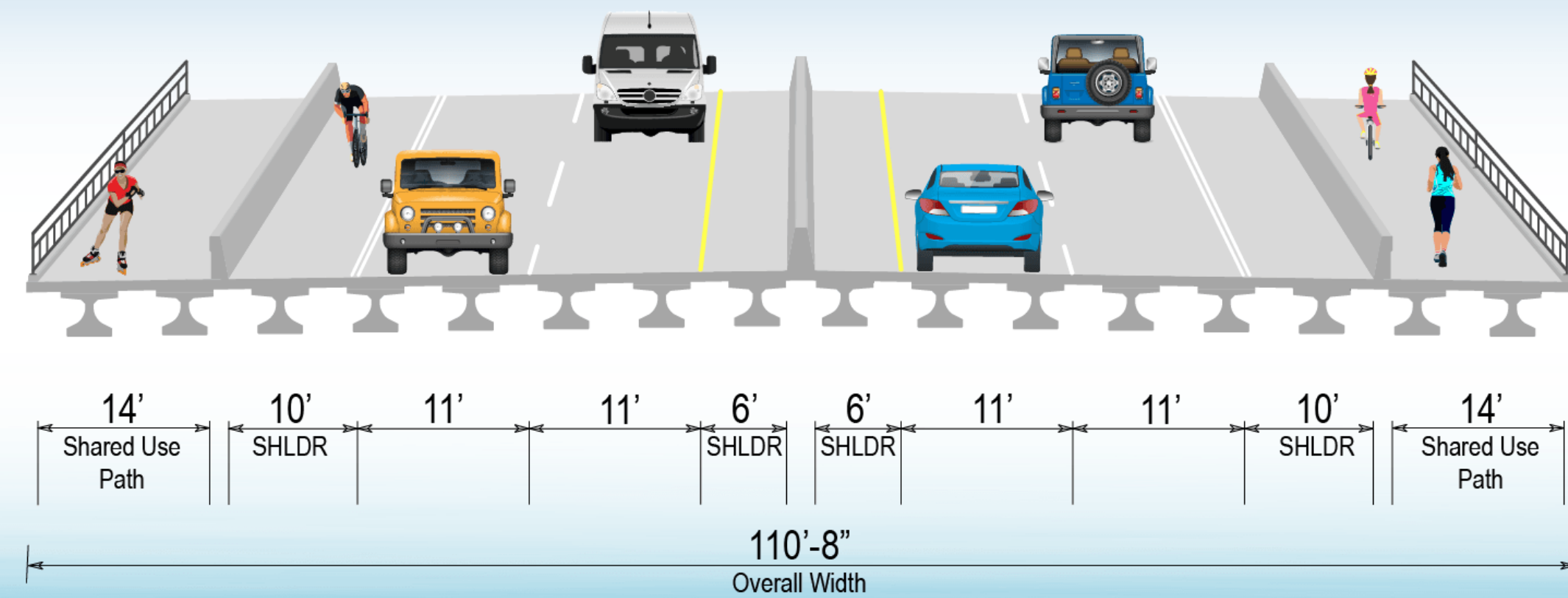
PROPOSED SINGLE BRIDGE TYPICAL SECTION
