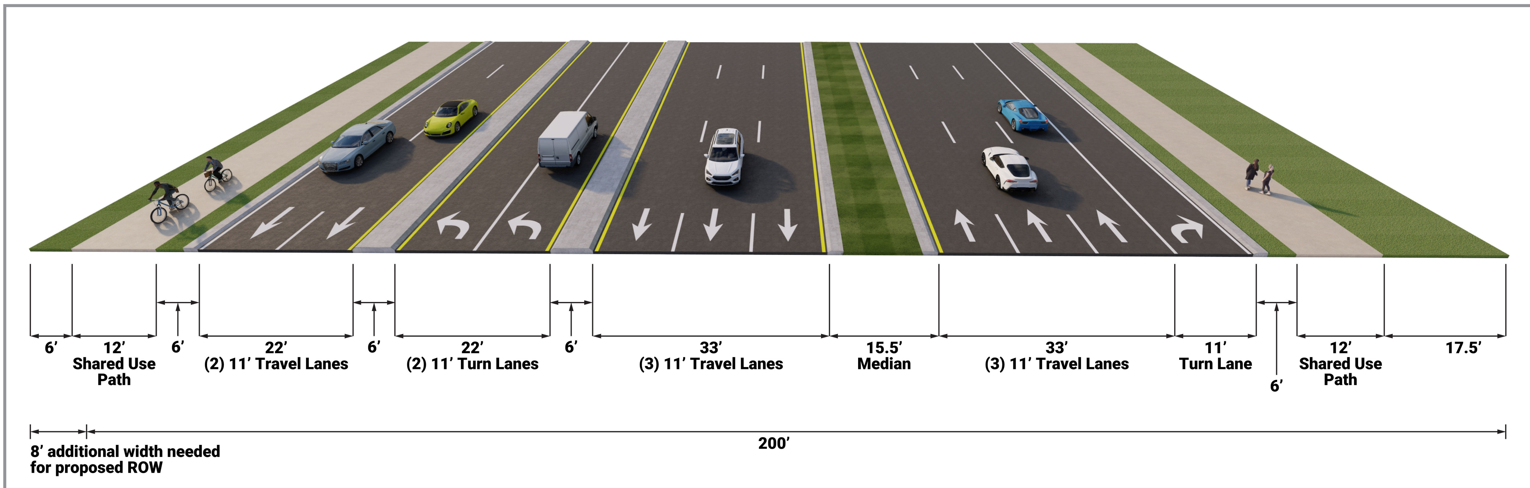
US 41 Displaced Left-Turn Intersection Proposed
