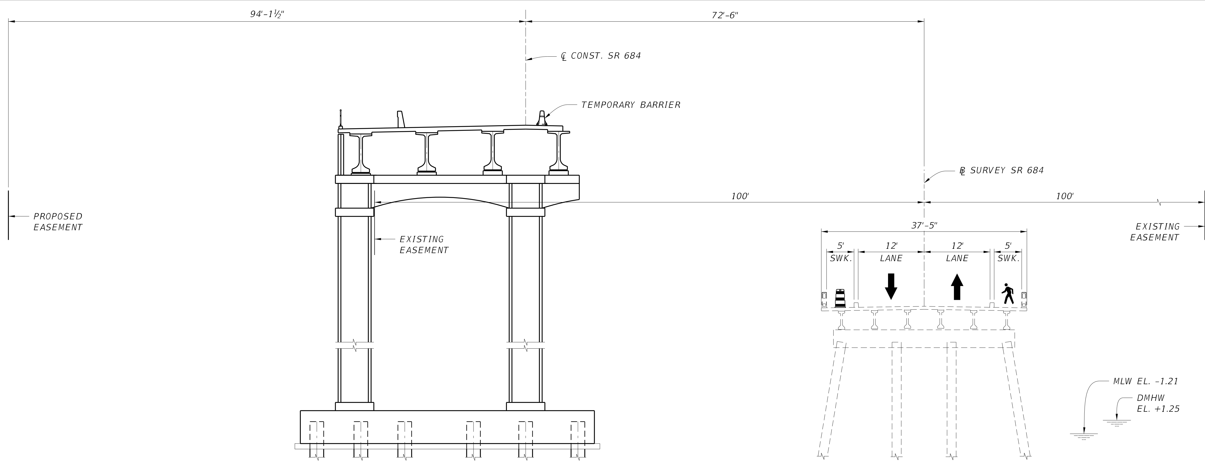
PHASE 1 (LOOKING EAST)
