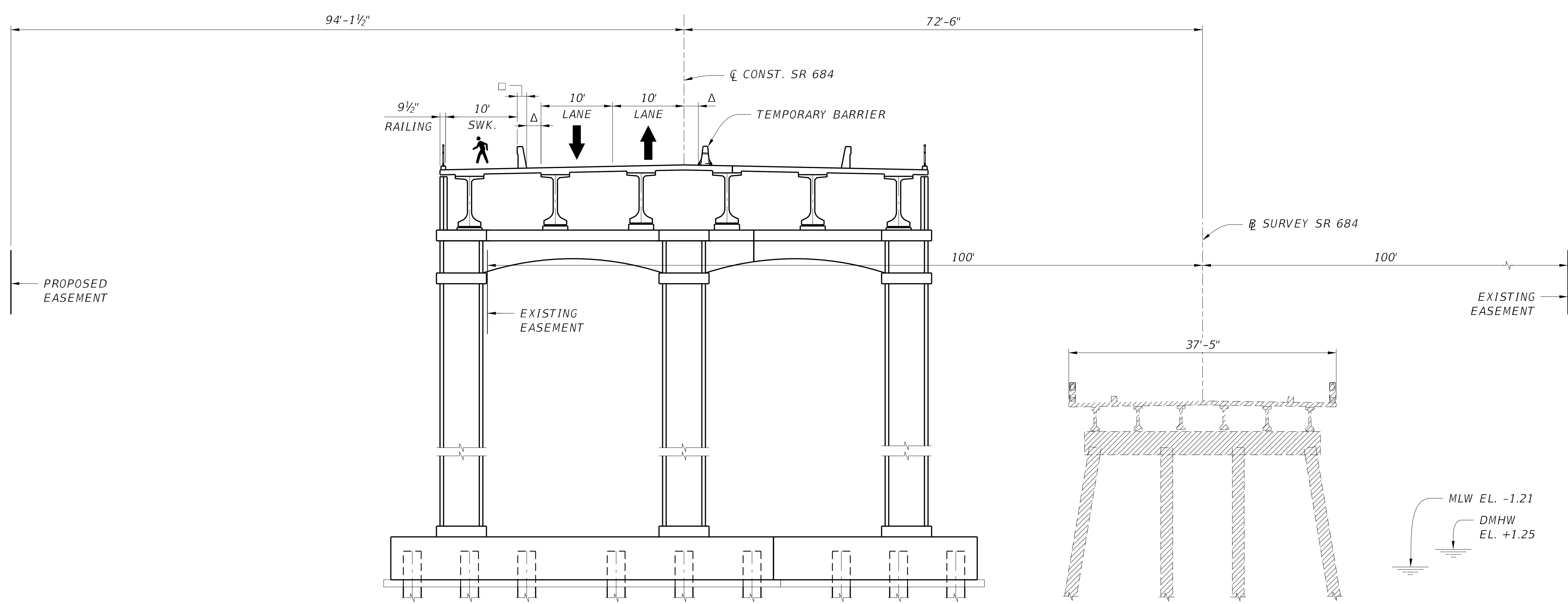
PHASE 2 (LOOKING EAST) ( \Delta = 2'-0" SHOULDER, \square = 1'-4" BARRIER)
