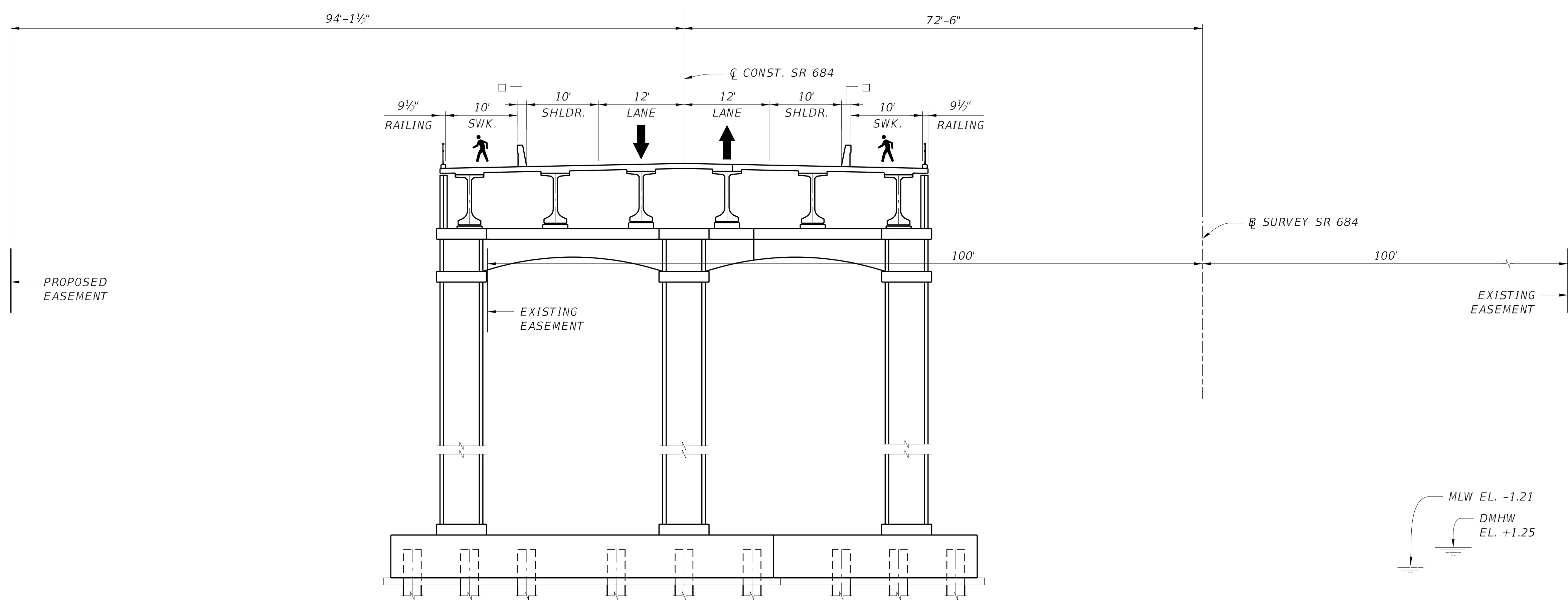
PHASE 3 & FINAL CONFIGURATION (LOOKING EAST) ( \square = 1'-4" BARRIER)
