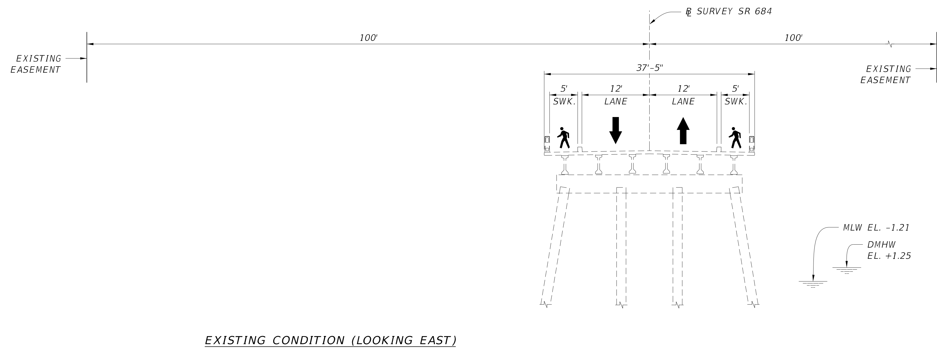
EXISTING CONDITION (LOOKING EAST)
