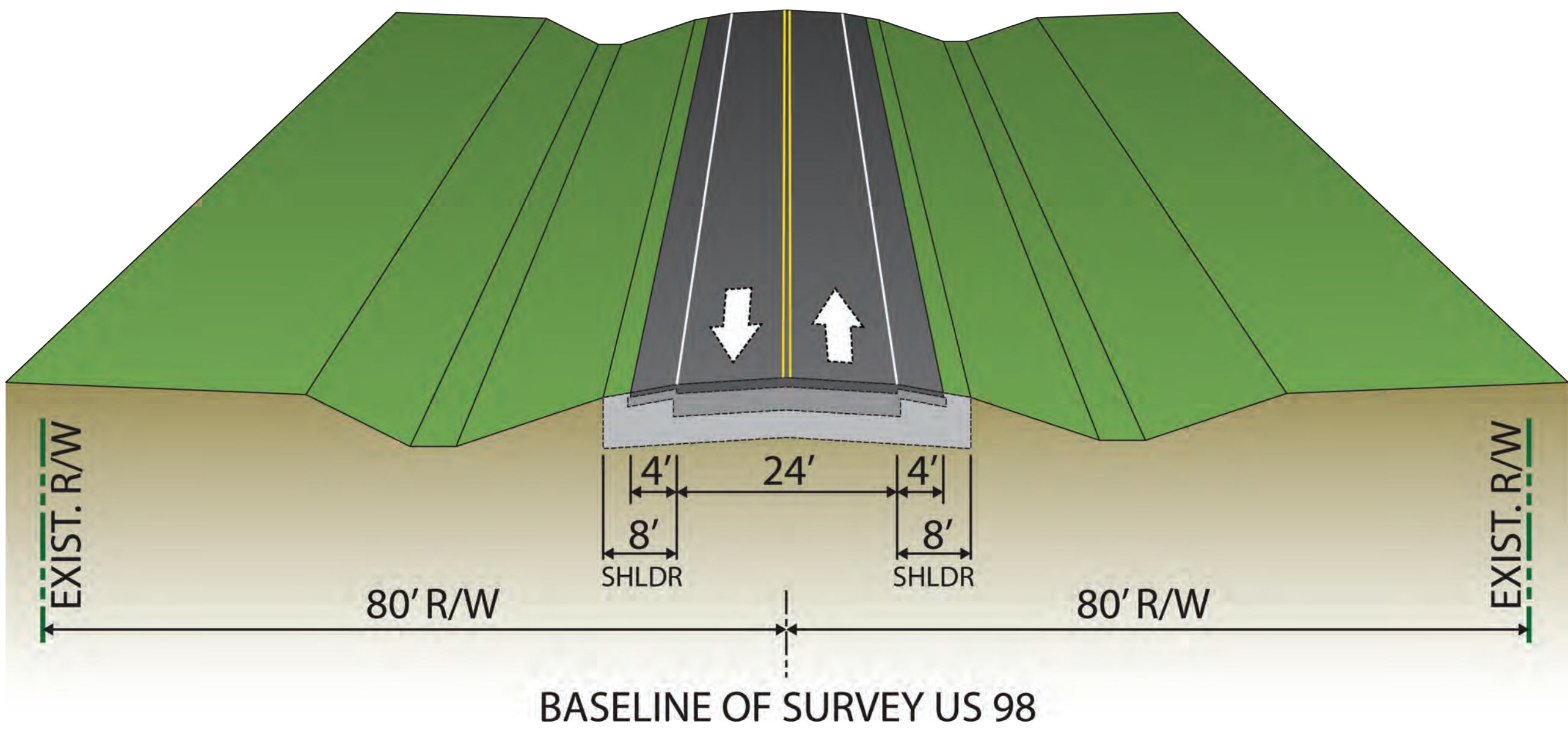
Existing US 98 Typical Section from North of West Socrum Loop Road to CR 54 60 mph Speed Limit
