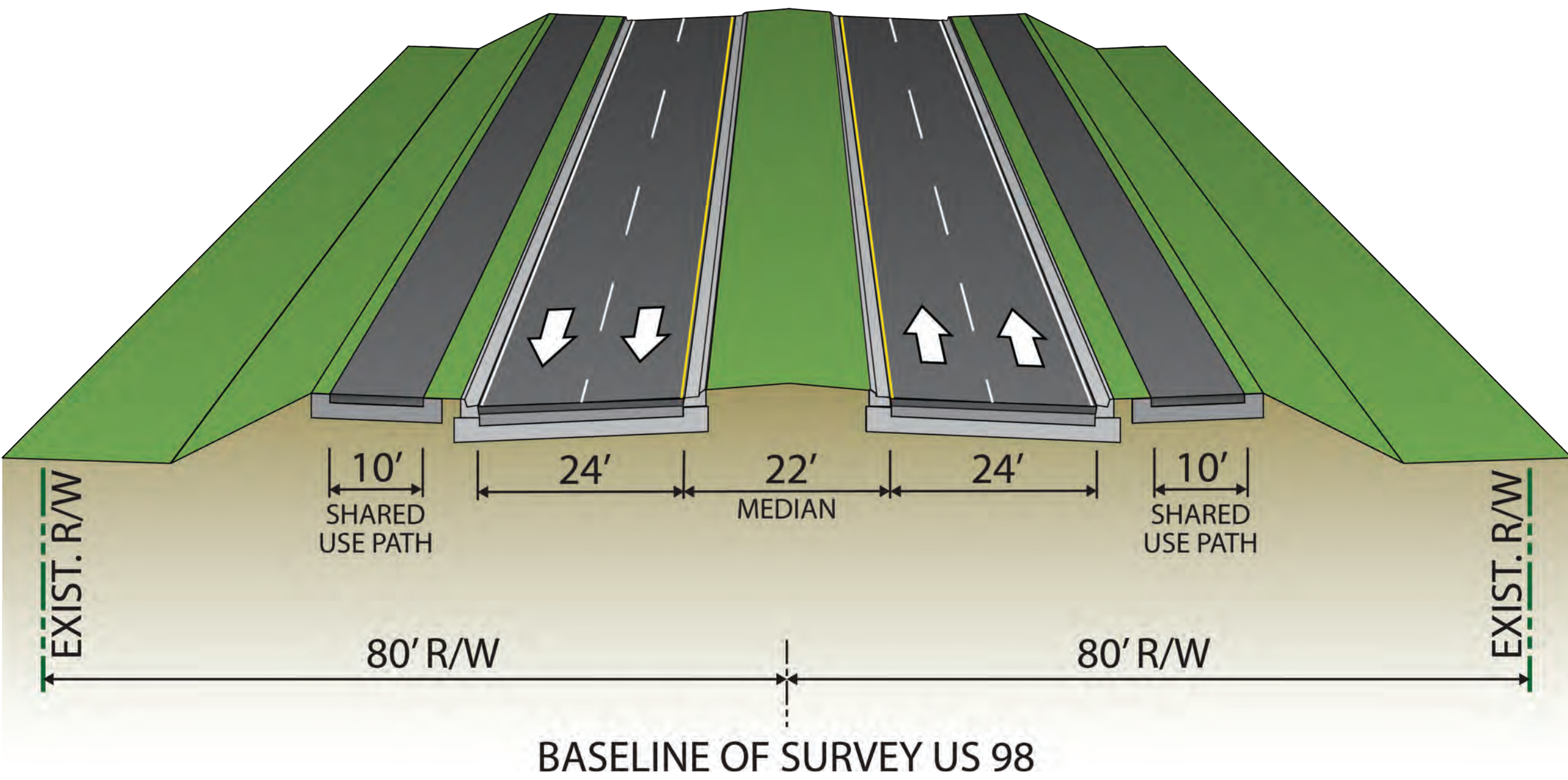
Proposed US 98 Typical Section from North of West Socrum Loop Road to North of Rock Ridge Road 45 mph Speed Limit
