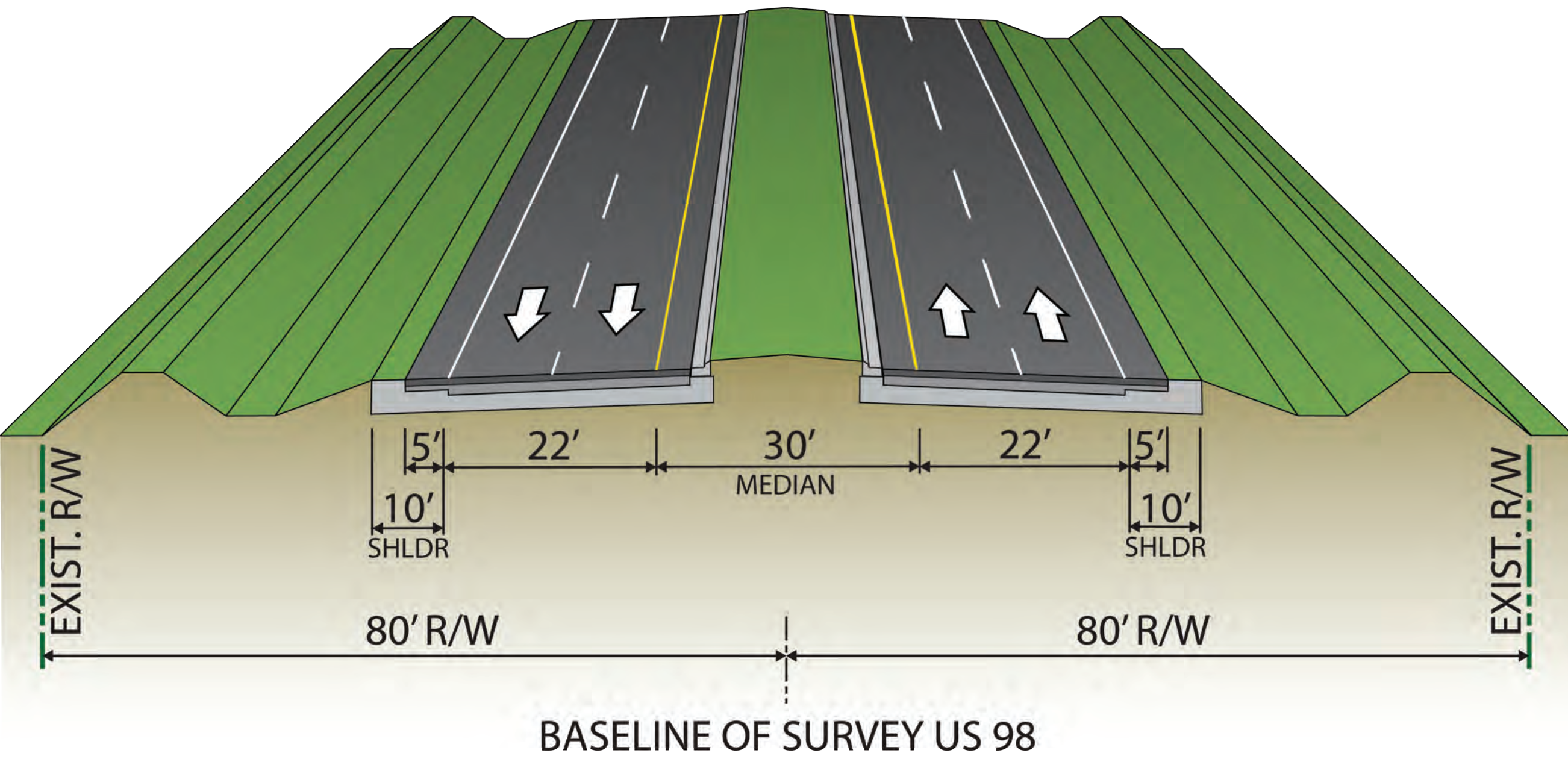
Proposed US 98 Typical Section from North of Rock Ridge Road to South of CR 54 55 mph Speed Limit
