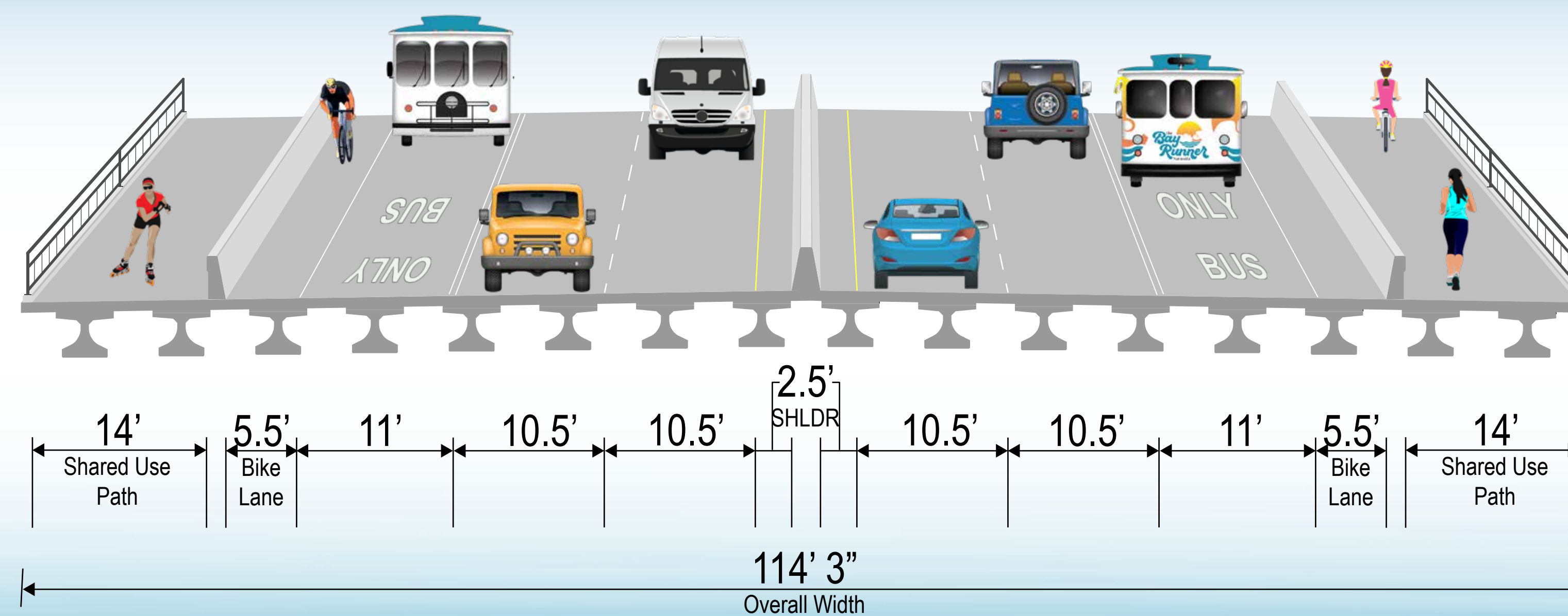
Single Bridge Typical
