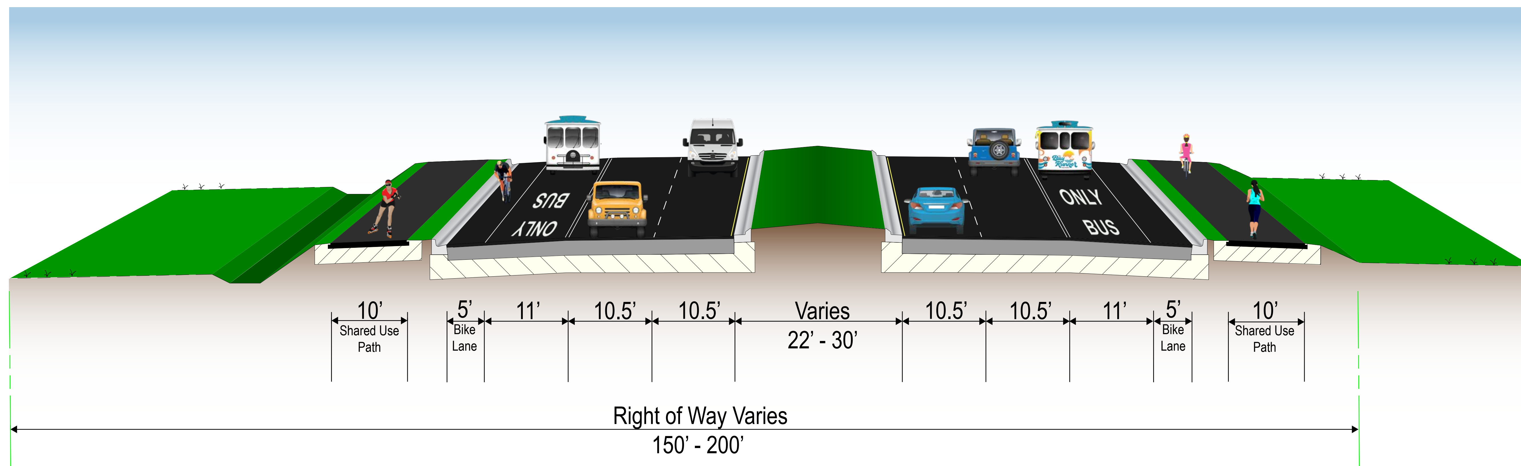
Roadway Typical
