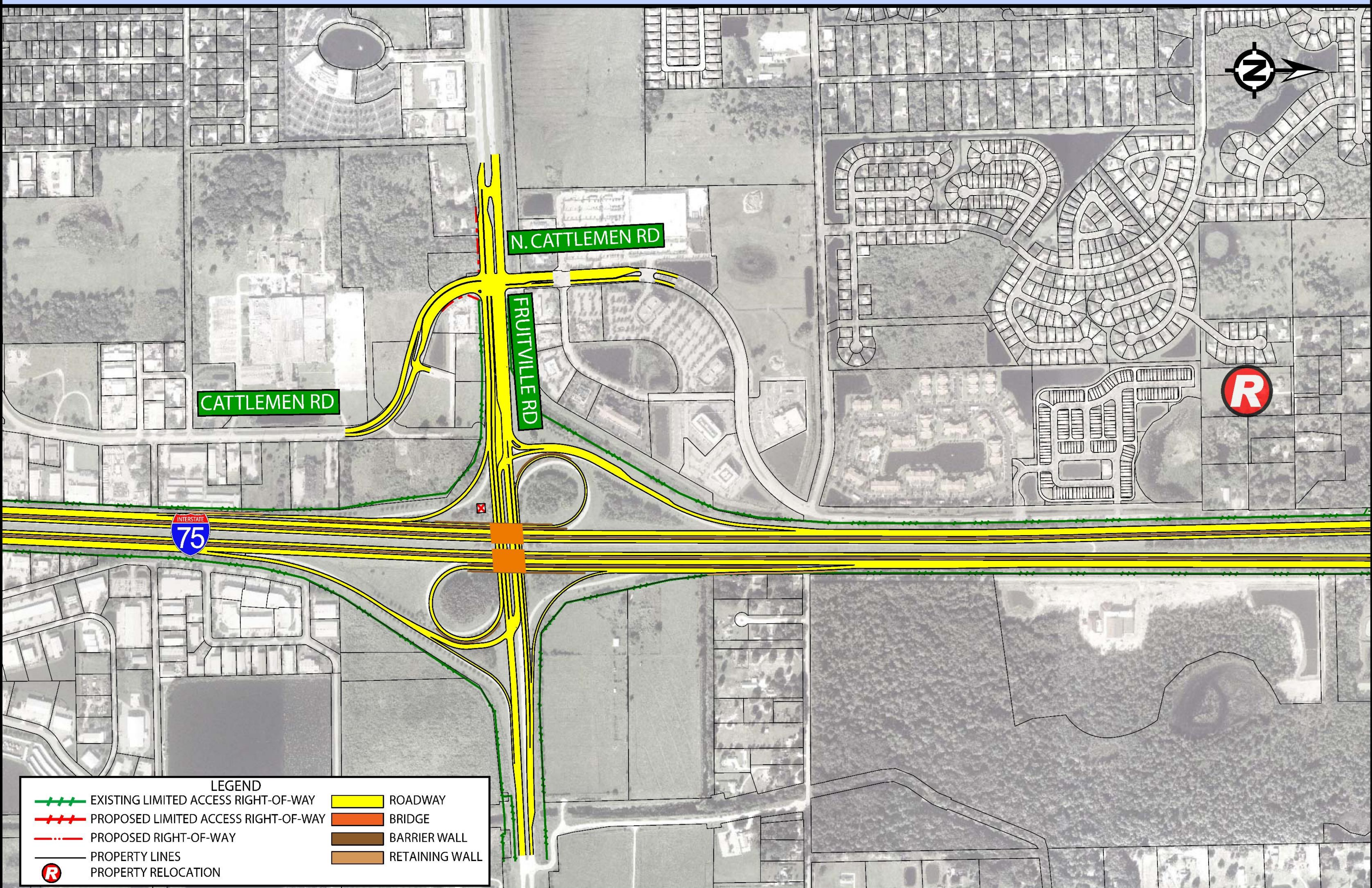
Figure 3-5 FRUITVILLE RD PREFERRED ALTERNATIVE
