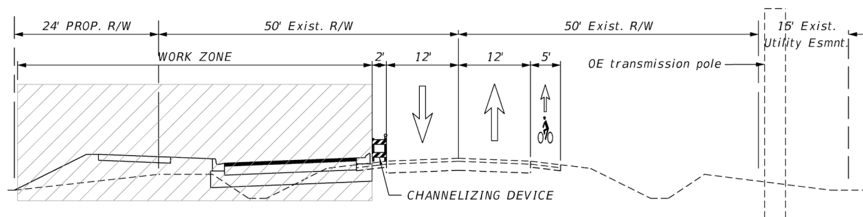
Figure 41: Phase 1 Typical Section
