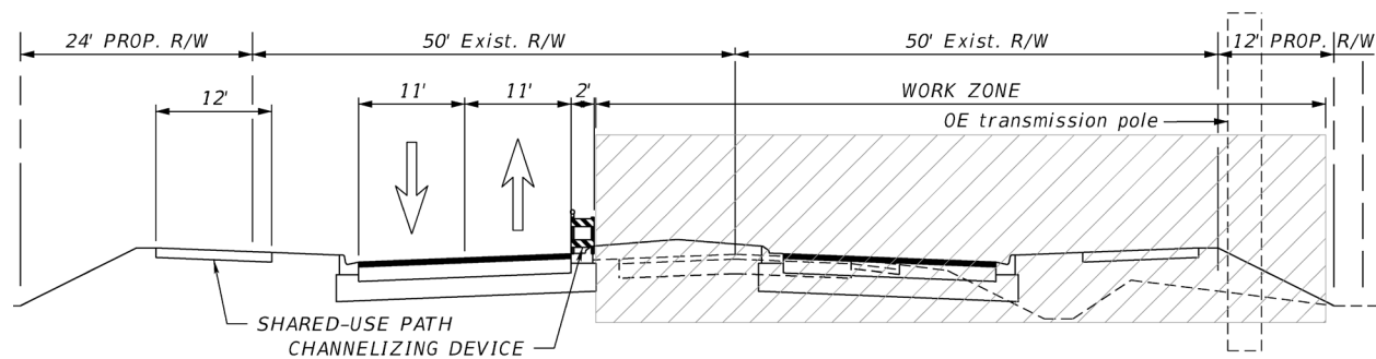
Figure 42: Phase 2 Typical Section
