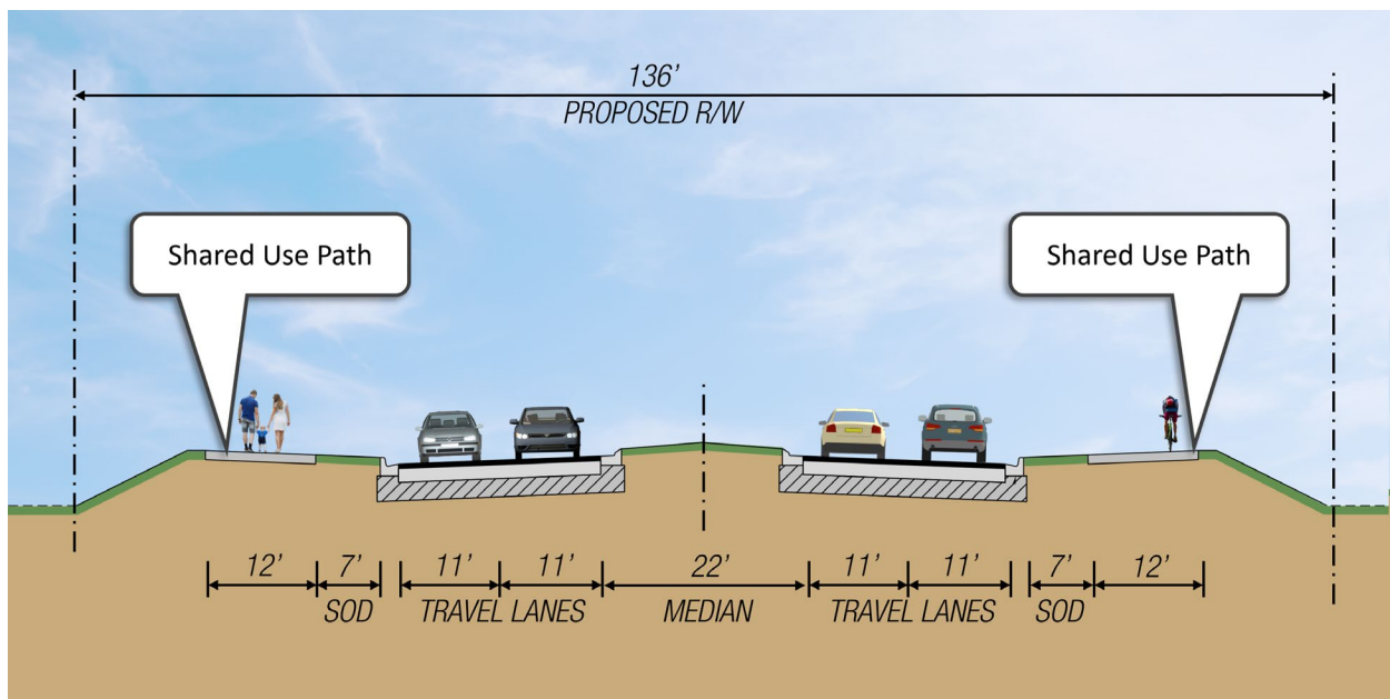
Figure 27: Proposed Typical Section SR 72
