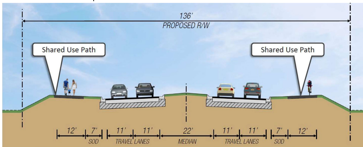
Figure 2: Preferred Alternative SR 72 Typical Section
