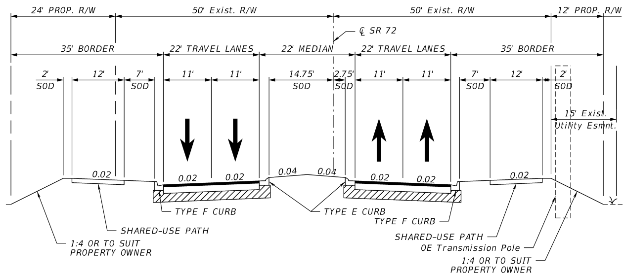
Figure 35: Proposed Typical Section for Segment 1, 2, and 4
