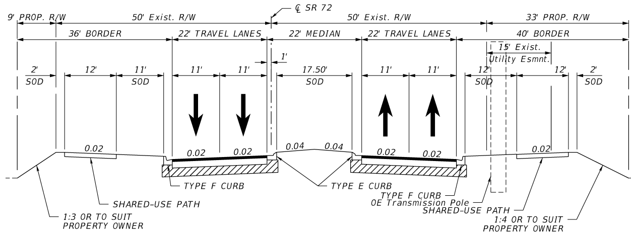
Figure 36: Proposed Typical Section for Segment 3
