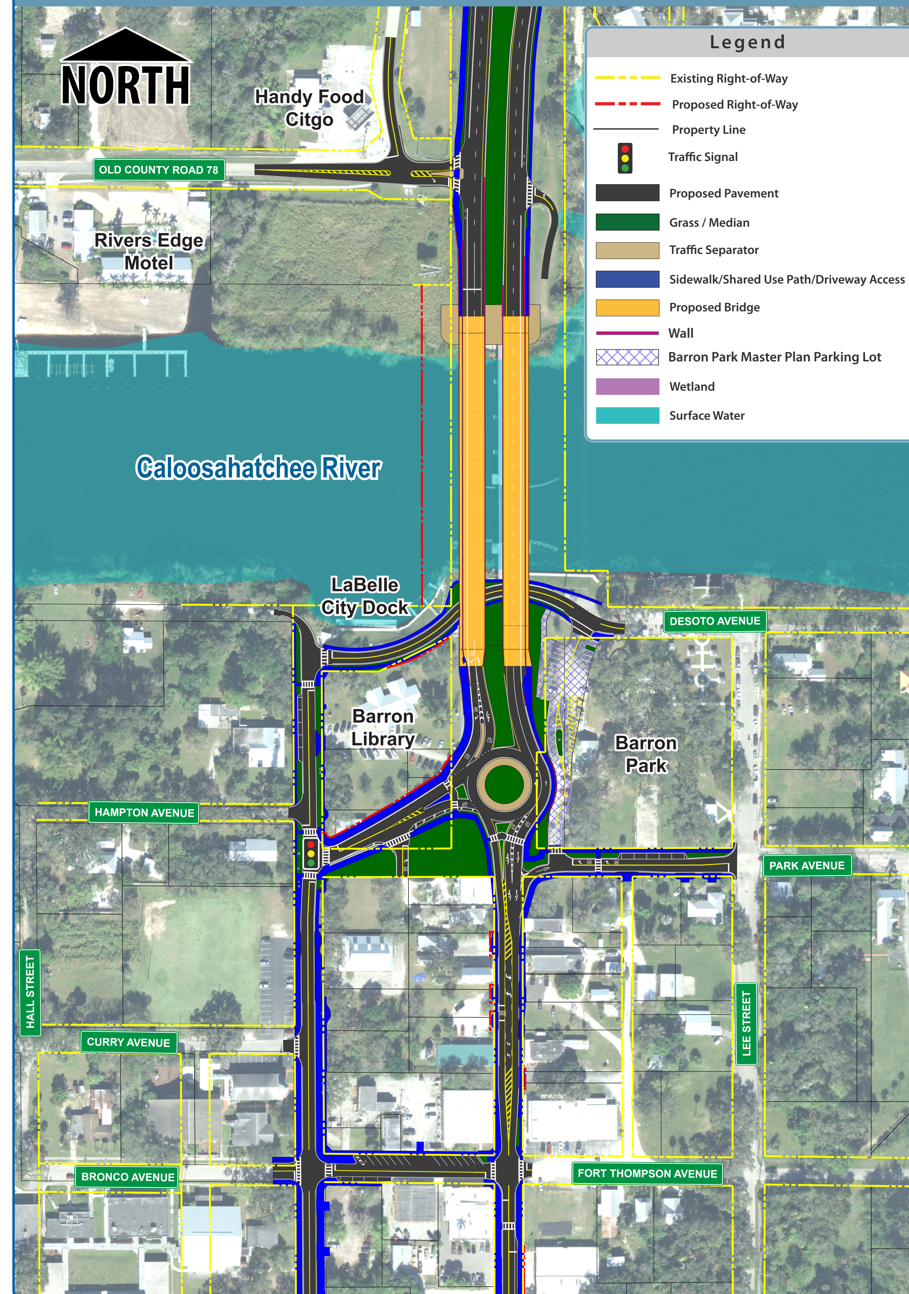
Roundabout Intersection 3C
