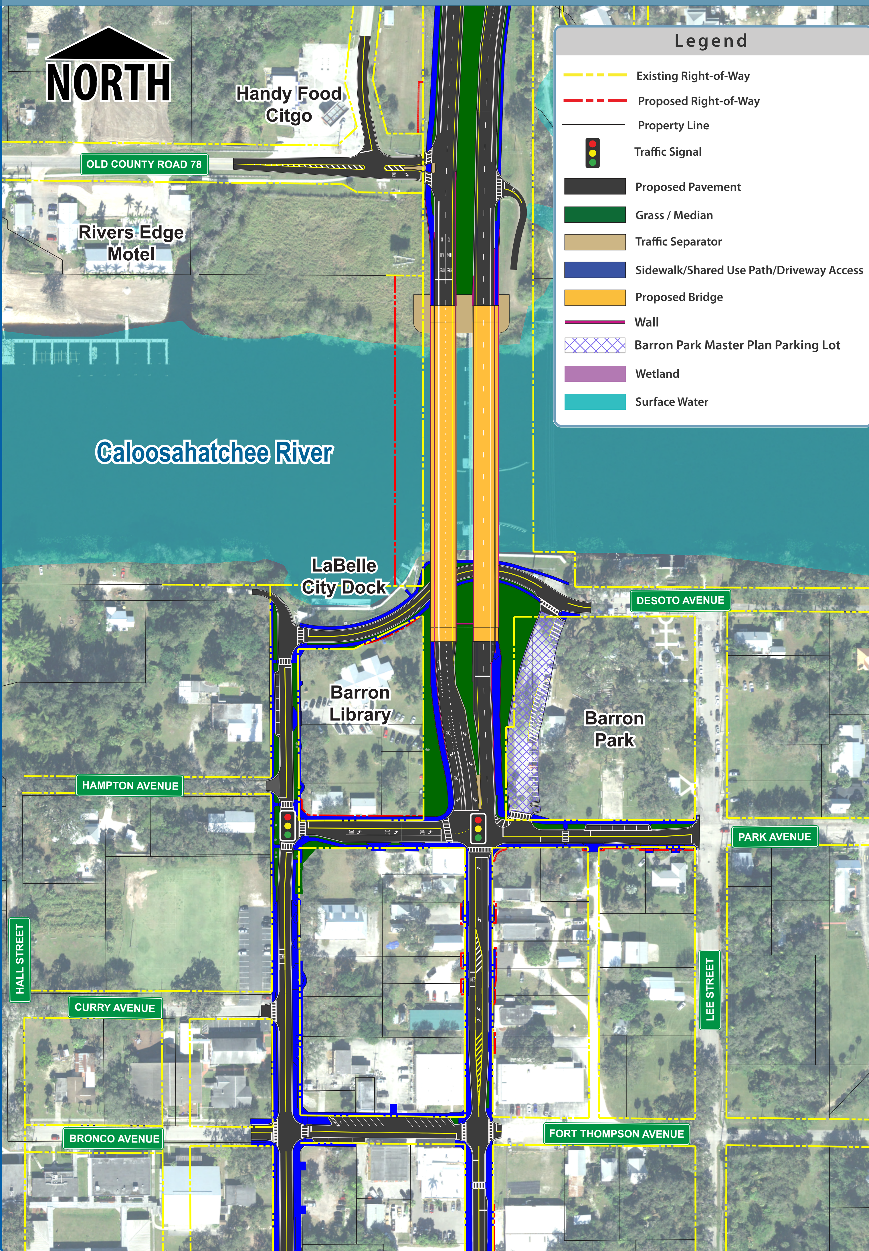
Conventional Signalized Intersection 3A
