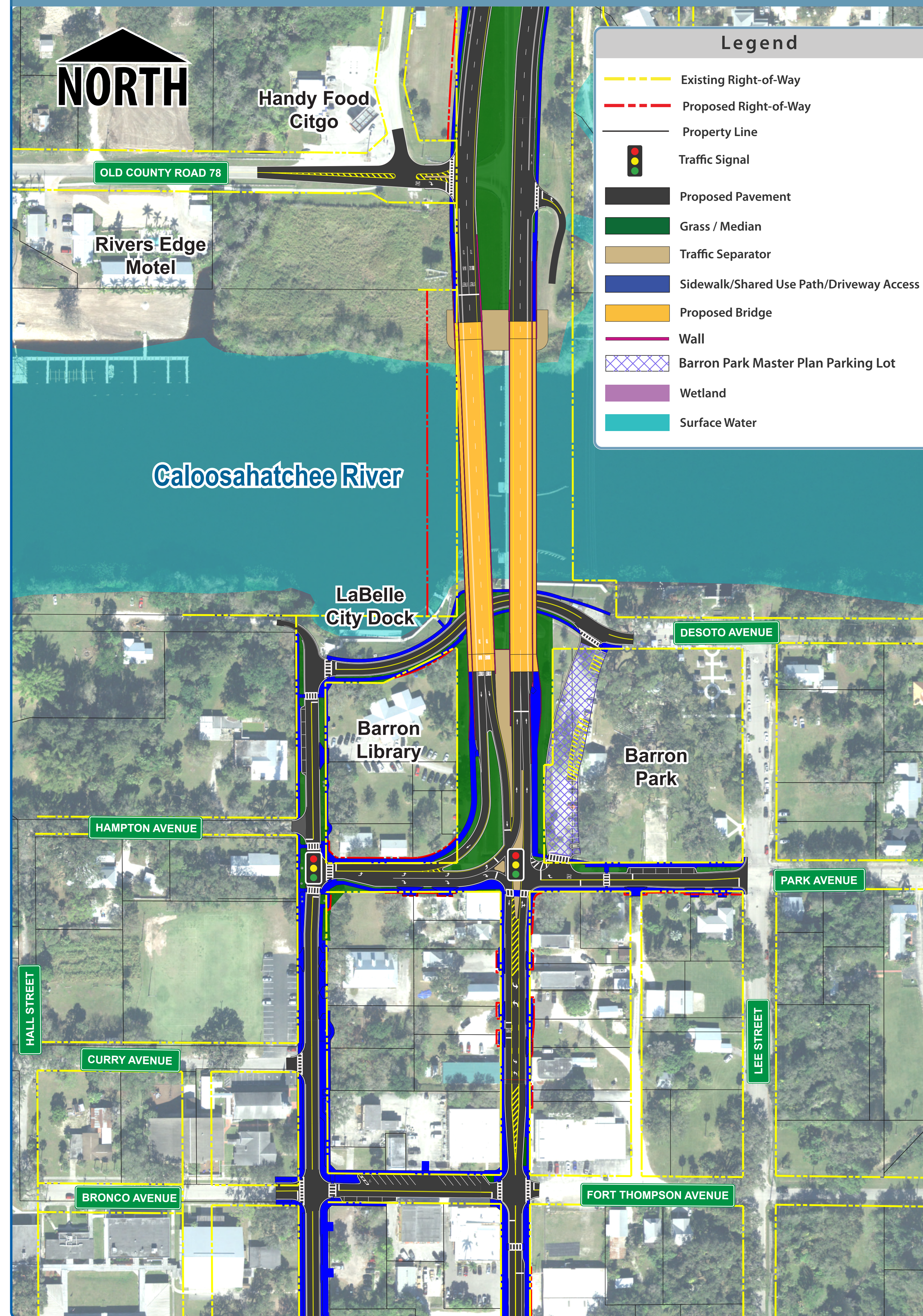
Signalized Florida T Intersection 3B
