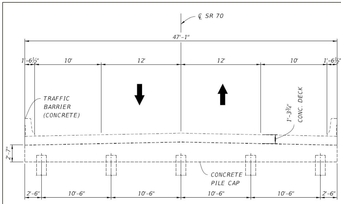
Figure 2-8 Existing Bridge Typical Section (Bridge No. 090053)
