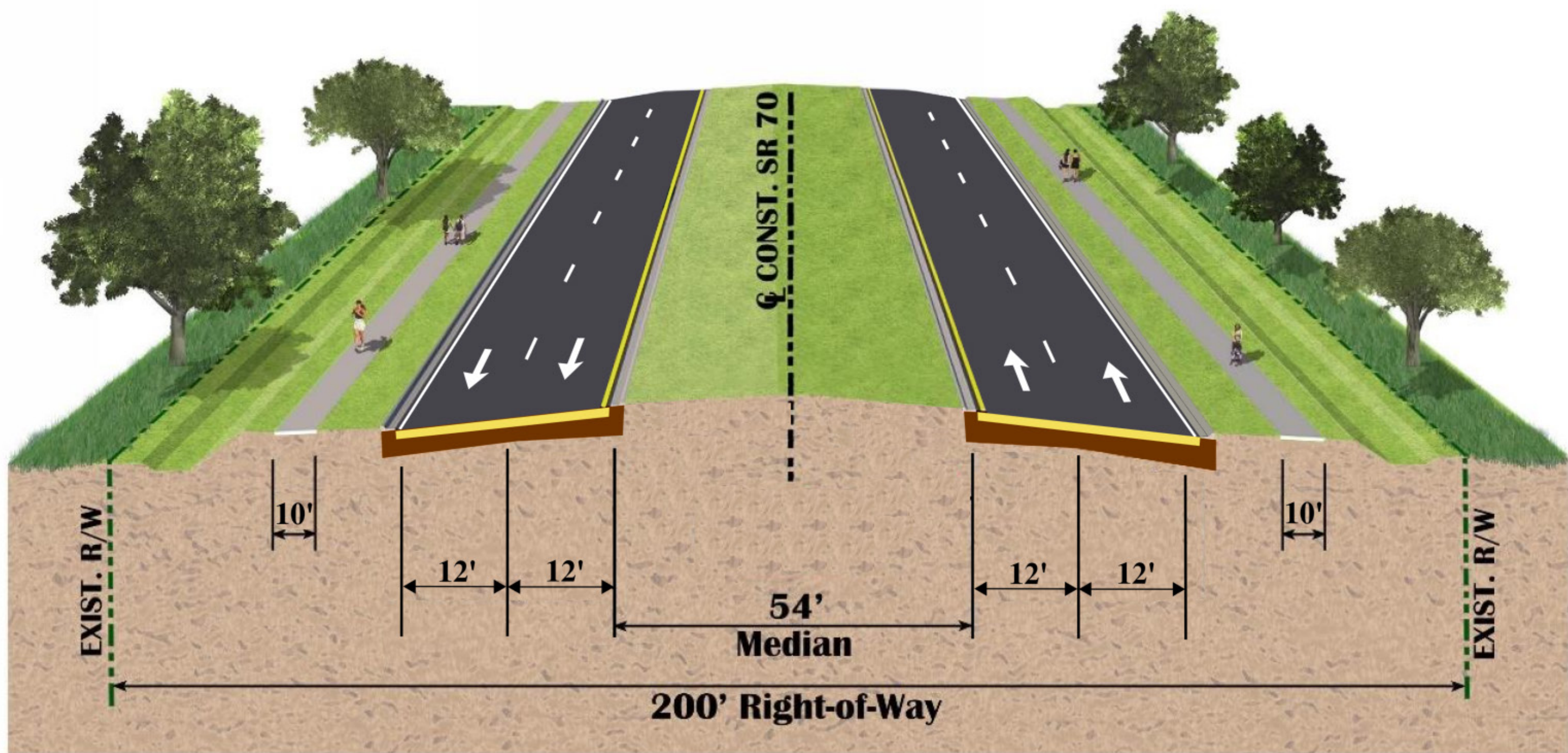
SR 70 from east of Greenbrook Boulevard to Bourneside Boulevard
