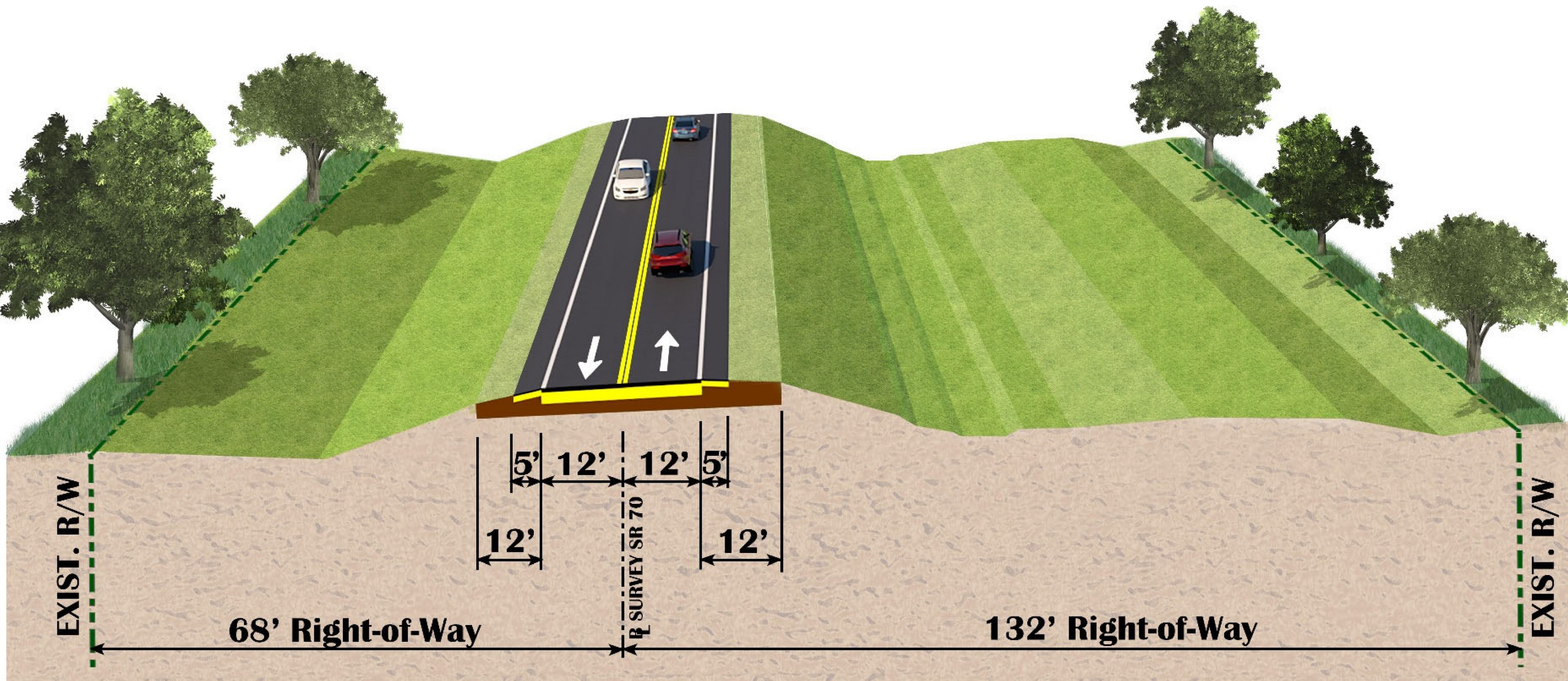
Existing Typical Section
