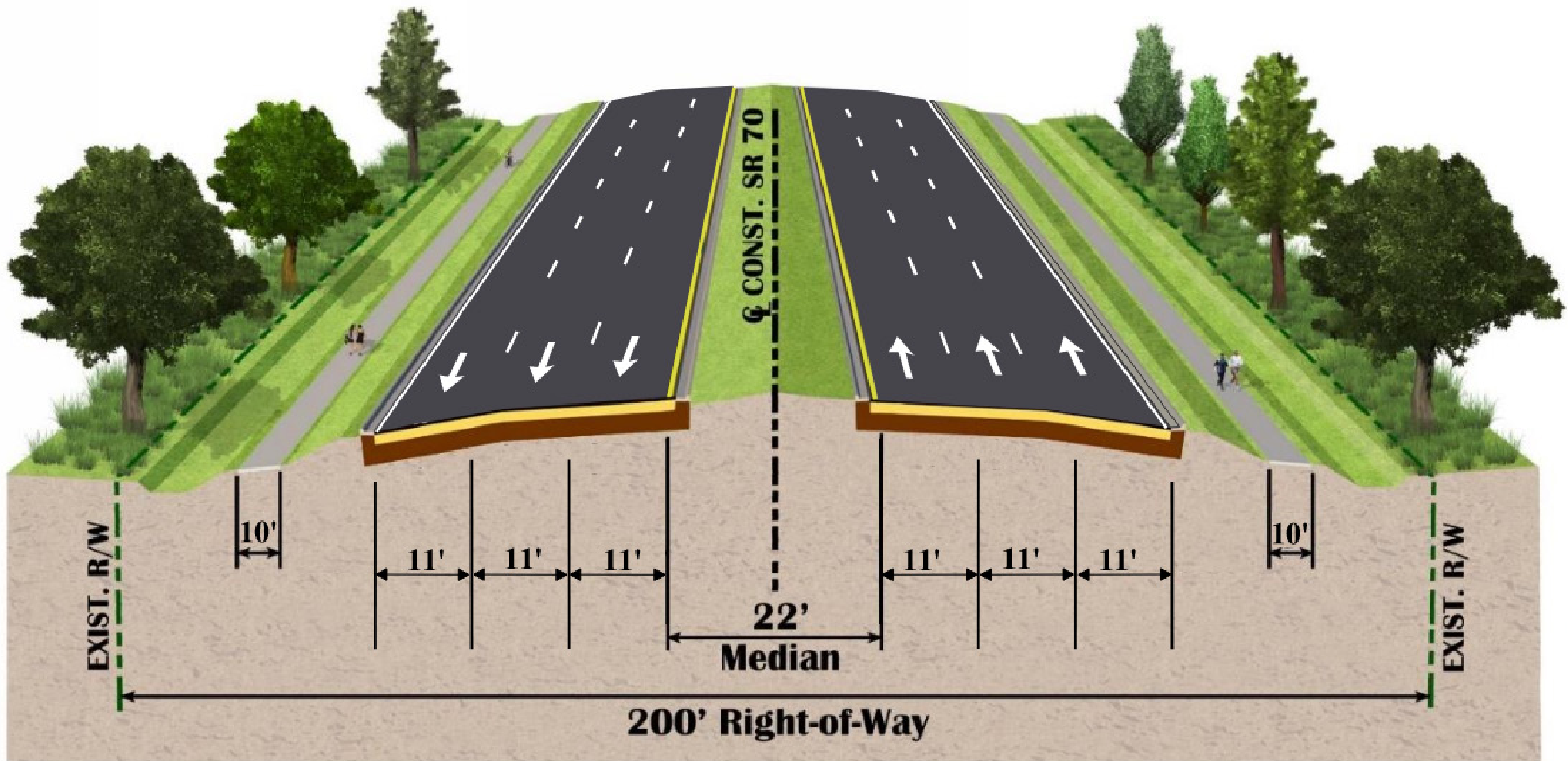
SR 70 from Lorraine Road to east of Greenbrook Boulevard
