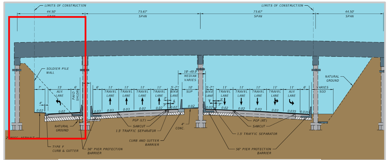
Typical Section- Daniels Parkway Looking East
