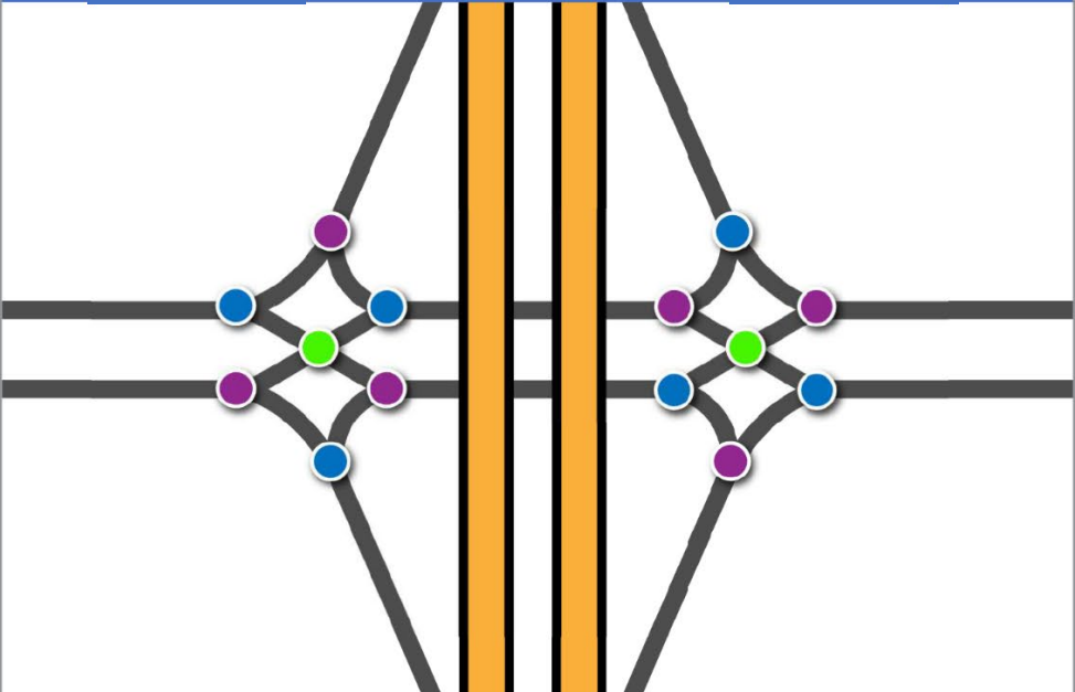
Diverging Diamond Interchange
