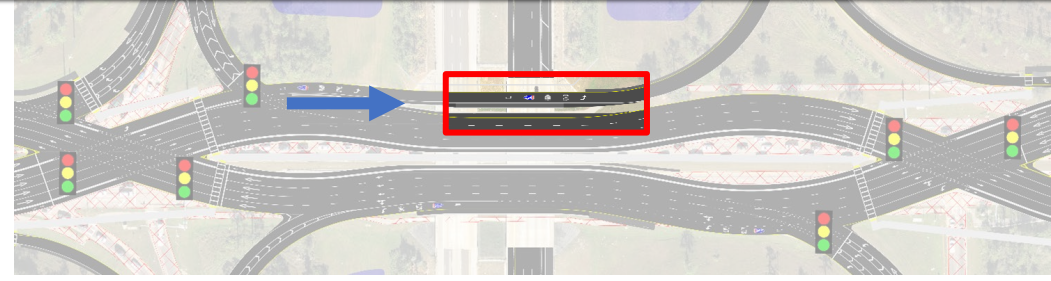
Splintered Typical Section- Daniels Parkway Looking East
