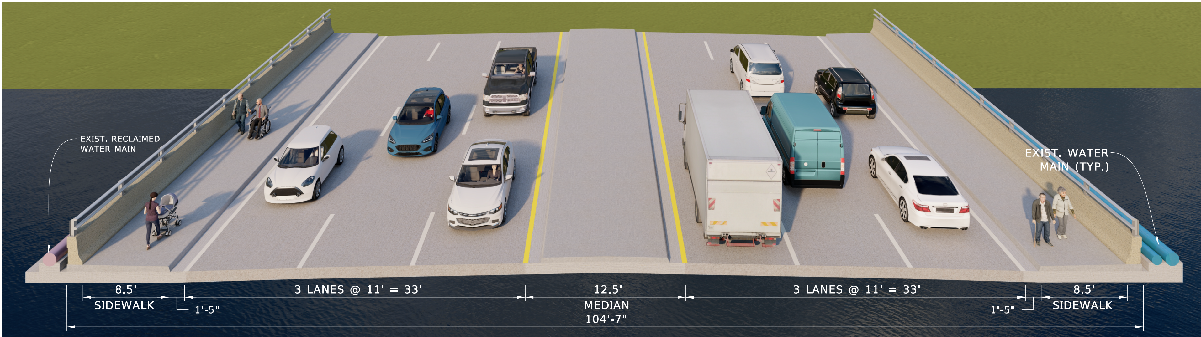
EXISTING TYPICAL SECTION (LIVINGSTON ROAD BRIDGE OVER GOLDEN GATE CANAL) (BRIDGE NO. 034060)
