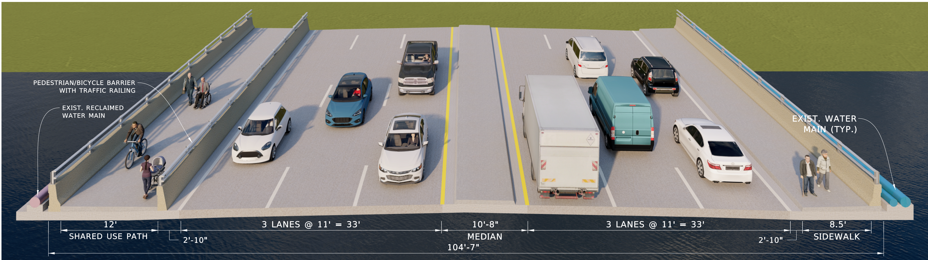
ALTERNATIVE 1 (LIVINGSTON RD) OPTION A - PROPOSED TYPICAL SECTION (LIVINGSTON ROAD BRIDGE OVER GOLDEN GATE CANAL) (BRIDGE NO. 034060)
