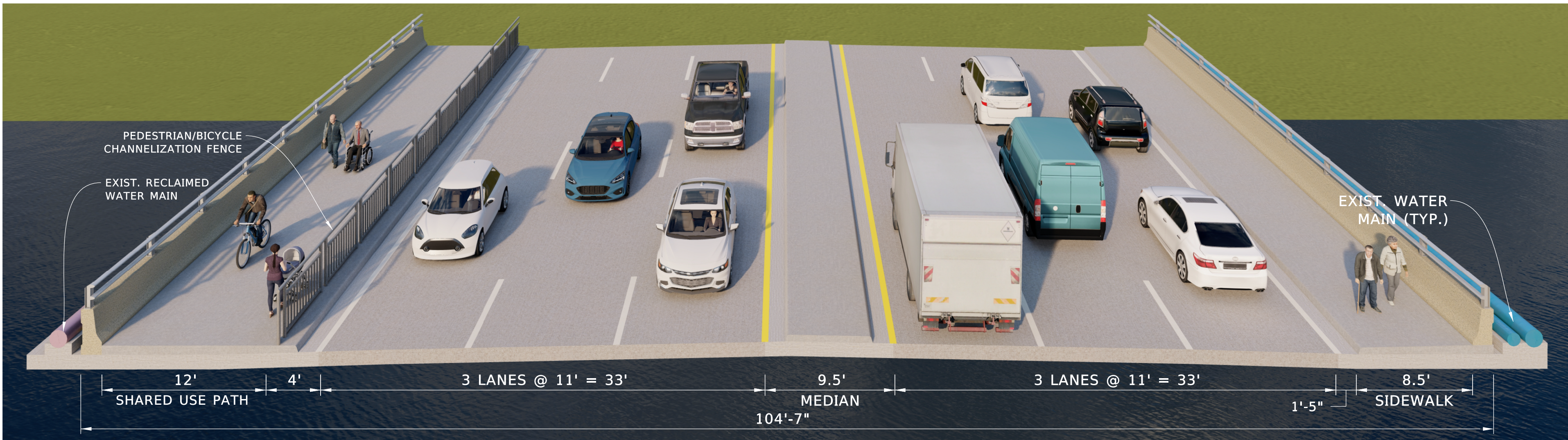
ALTERNATIVE 1 (LIVINGSTON RD) OPTION B - PROPOSED TYPICAL SECTION (LIVINGSTON ROAD BRIDGE OVER GOLDEN GATE CANAL) (BRIDGE NO. 034060)
