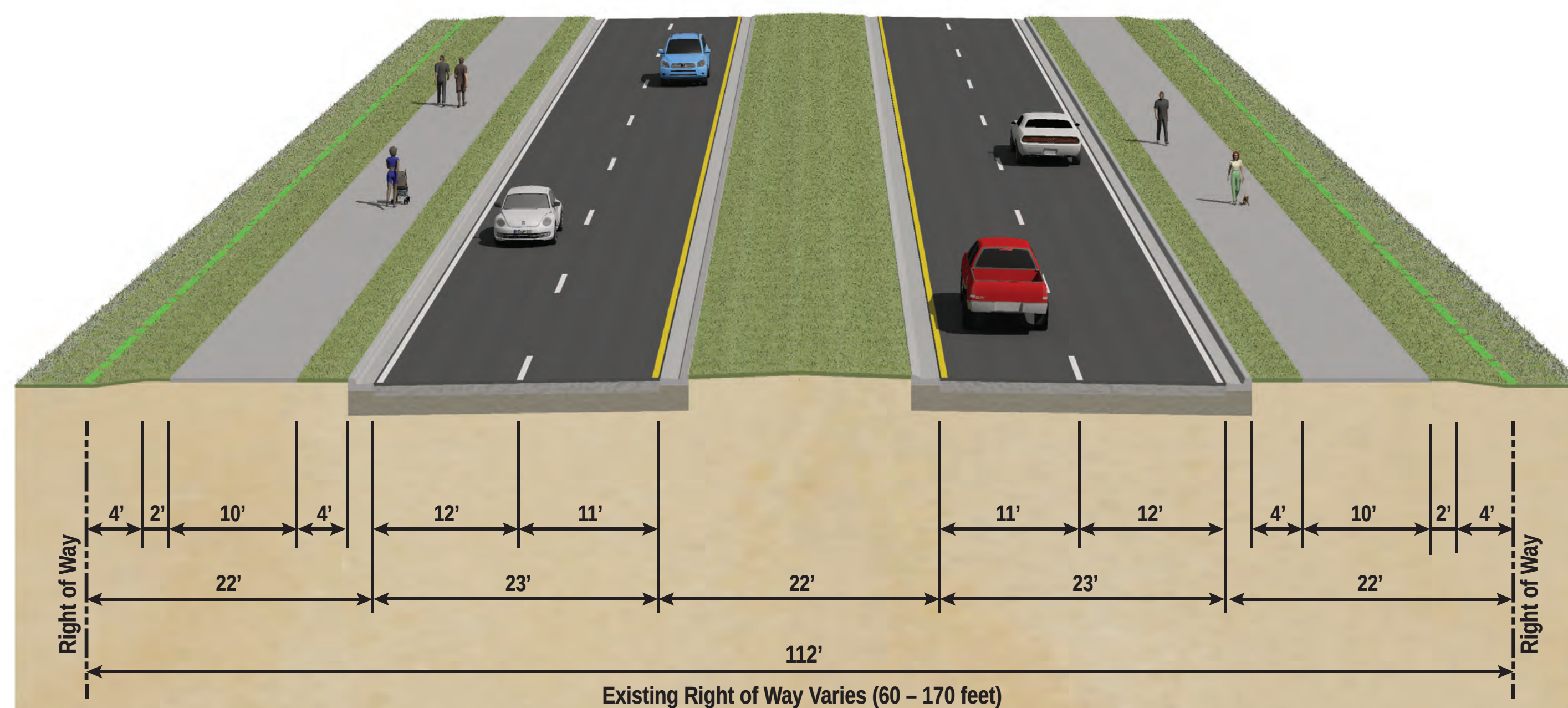
Four Lane Urban Divided Roadway
